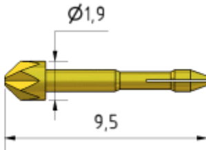
Kopfform/Tip style No. 14
