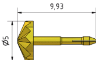
Kopfform/Tip style No. 14
