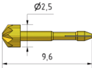
Kopfform/Tip style No. 14
