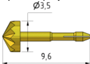
Kopfform/Tip style No. 14
